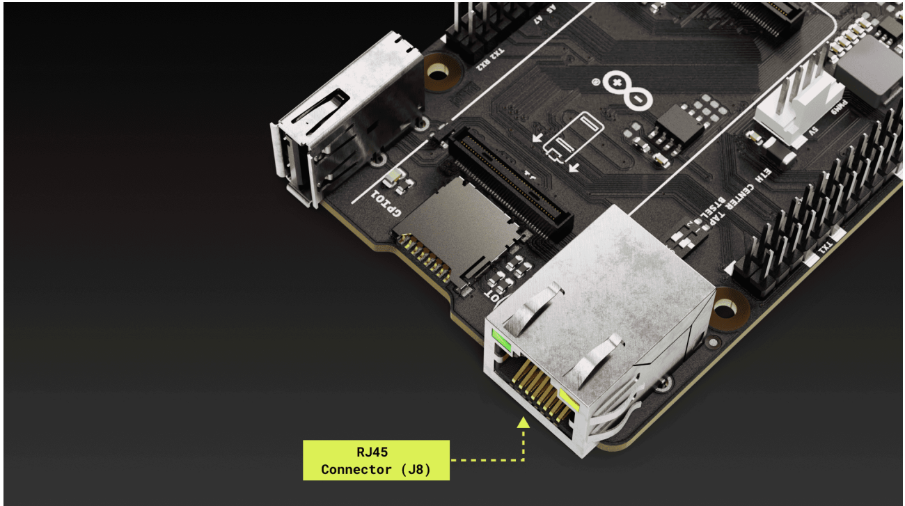
Figure 11. RJ45 connector of the Portenta Hat Carrier
