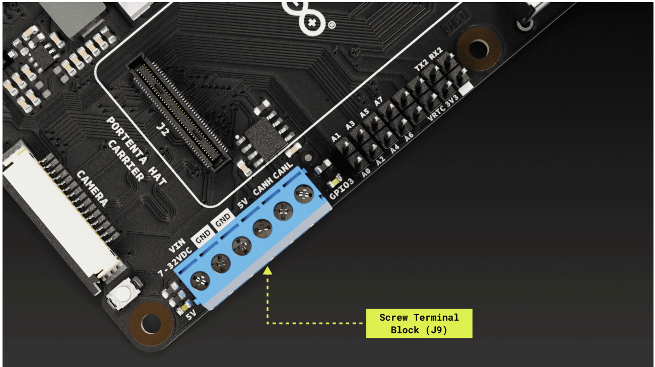
Figure 12. Screw terminal block connector of the Portenta Hat Carrier
